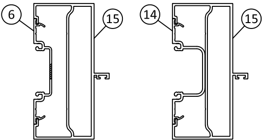
TYPE 'M1' NO REINFORCING
