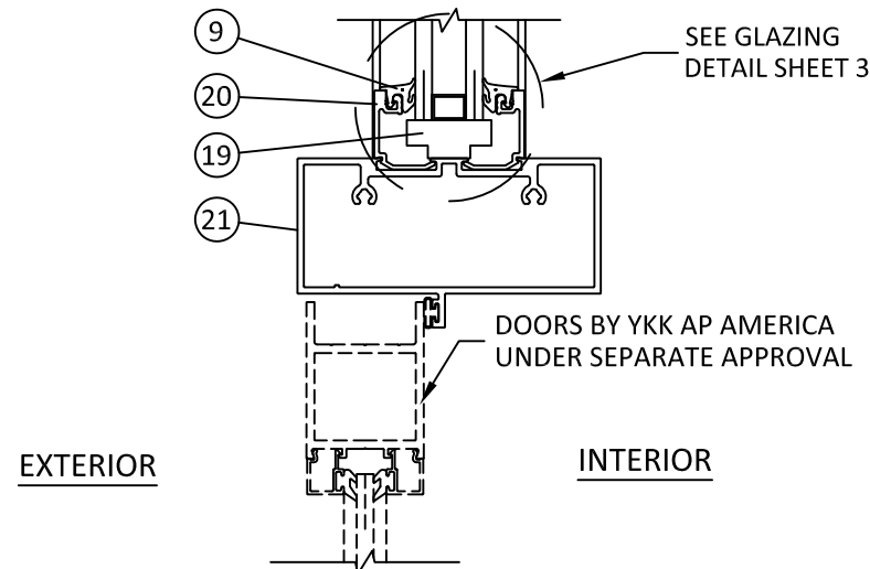
T 9 VERTICAL SECTION DOOR HEAD W/ TRANSOM
