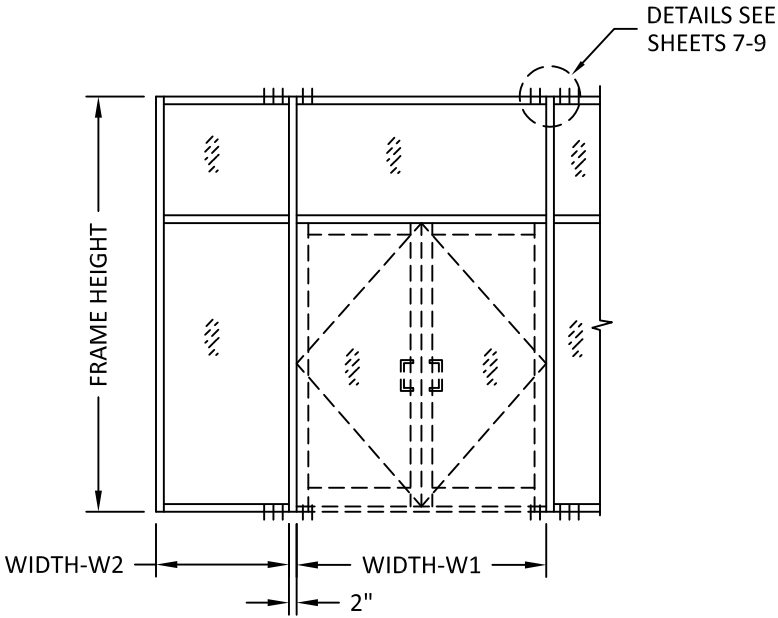
DOUBLE DOOR W/ TRANSOM
