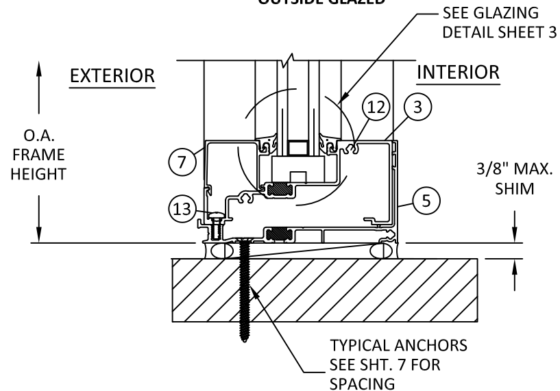
C 8 VERTICAL SECTION SILL - INSIDE/OUTSIDE GLAZED IF MULLION END LOAD REACTION IS OVER 500 LBS (INSIDE GLAZED), USE THIS SILL CONDITION.
