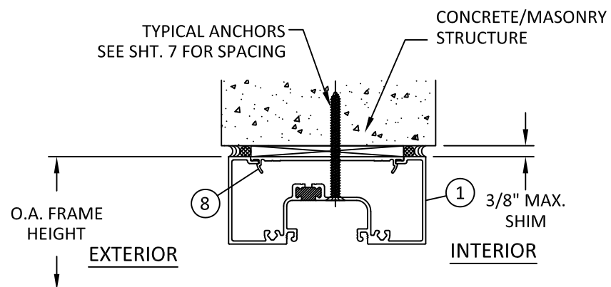
E 8 VERTICAL SECTION HEAD - CONCRETE/MASONRY
