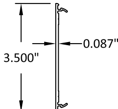
8 SNAP IN COVER
