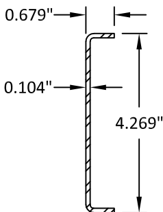
16 DOOR MULLION REINFORCING CHANNELS
