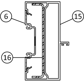
TYPE 'M2' LIGHT REINFORCING
