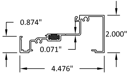
3 SILL (I.G. / O.G.) HEAD (I.G.)
