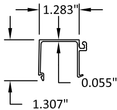
7 GLAZING STOP
