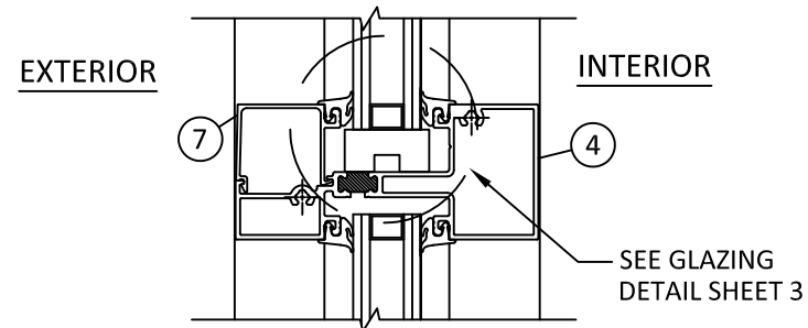
B 8 VERTICAL SECTION HORIZONTAL MEMBER OUTSIDE GLAZED
