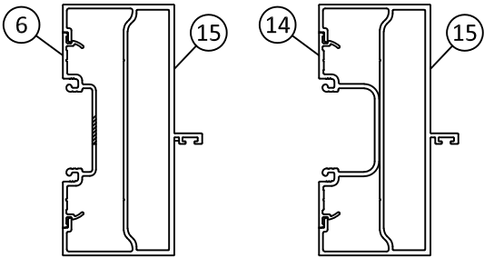
NO REINFORCING
